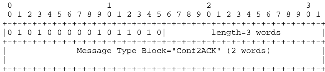
Figure 11: Conf2ACK Message Format
