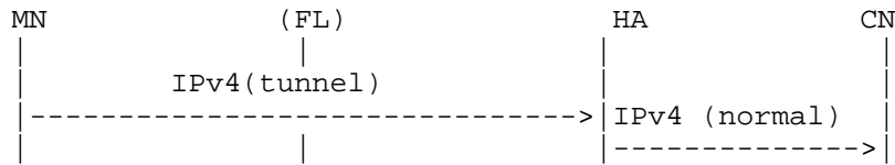
(c) MIPv4: MN-->CN, the reverse tunnel with co-located CoA
