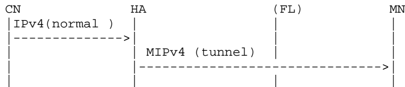
(e) MIPv4: CN-->MN with co-located CoA
