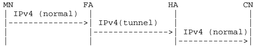
(b) MIPv4: MN-->CN, the reverse tunnel with FA CoA
