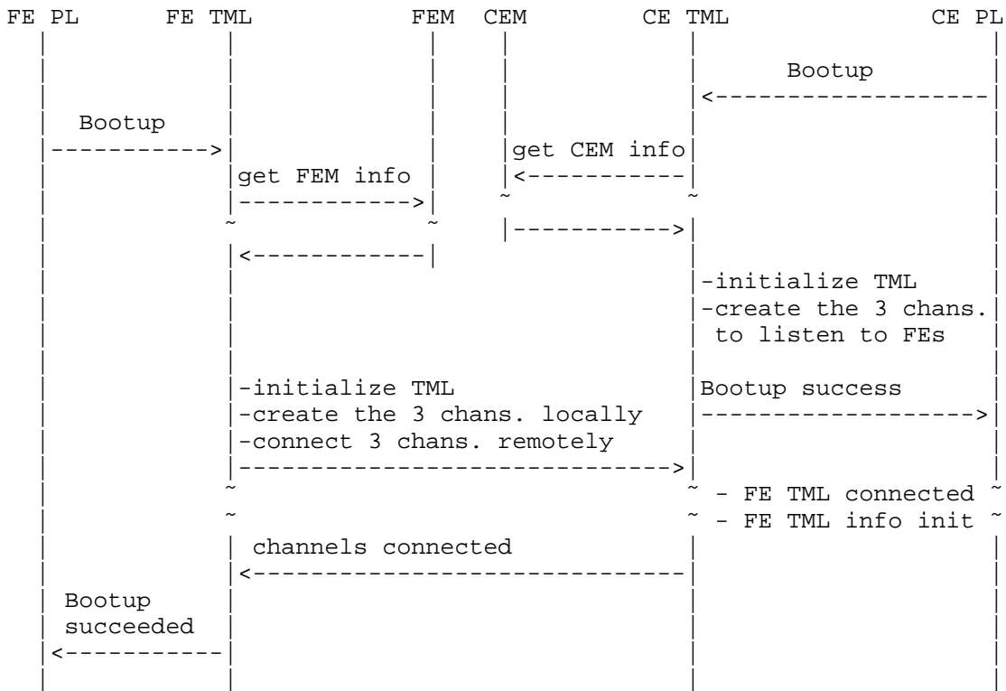
Figure 6: SCTP TML Bootstrapping
