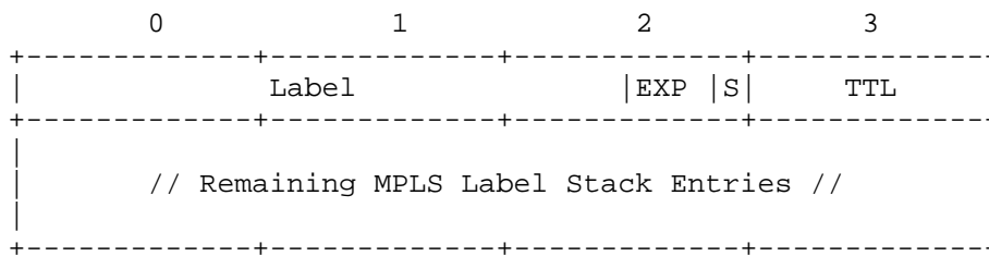
Figure 2: MPLS Label Stack Object
