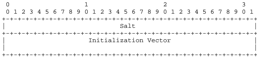
Figure 2: Nonce Format
