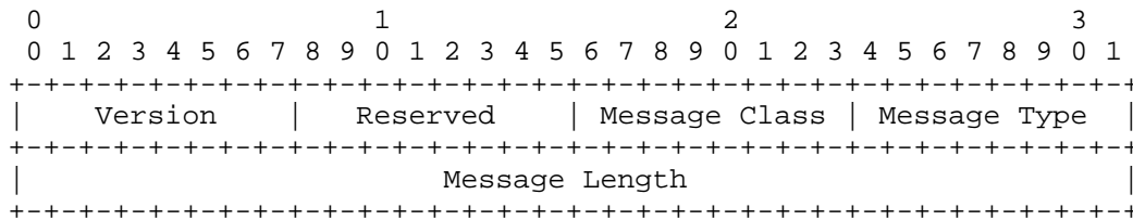
Figure 3 Common Header Format
