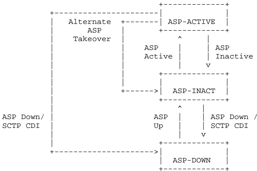
Figure 7 ASP State Transition Diagram
