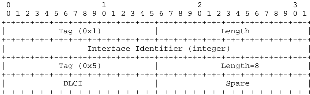
Figure 4 IUA Message Header (Integer-based Interface Identifier)
