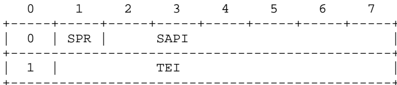
Figure 6 DLCI Format
