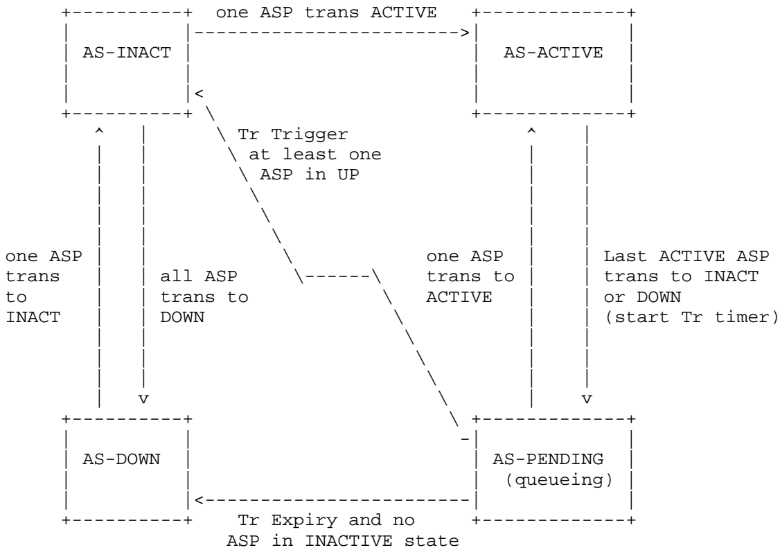
Figure 8 AS State Transition Diagram
