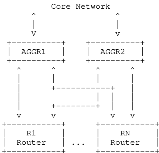
Figure 1: Reference Dual Hub-and-Spoke Topology
