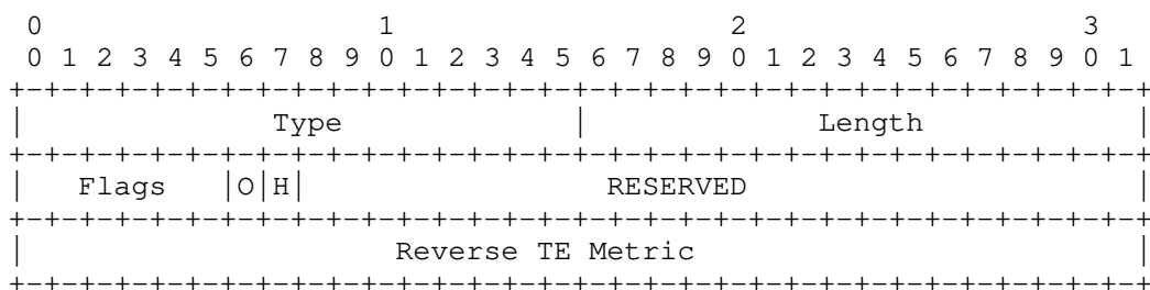
Figure 3: Reverse TE Metric TLV
