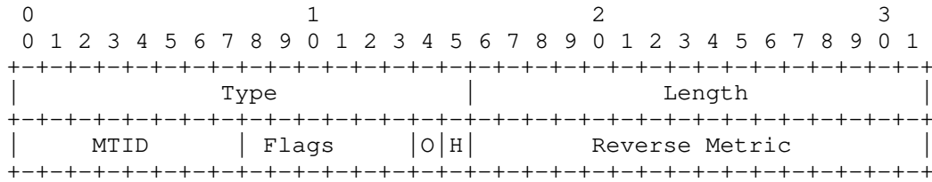
Figure 2: Reverse Metric TLV
