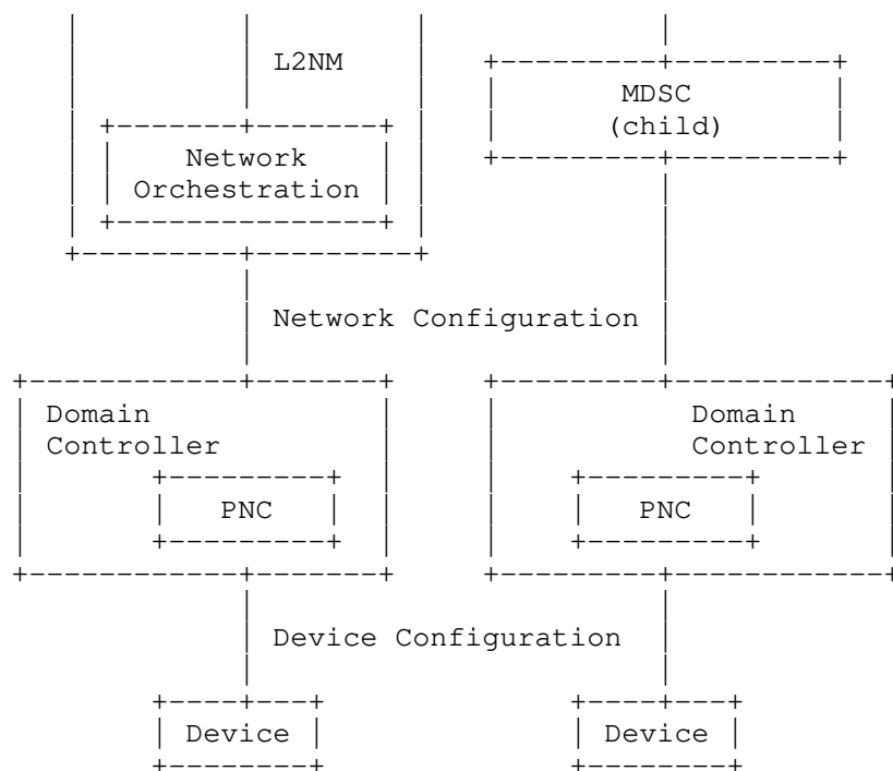
Figure 2: L2SM and L2NM in the Context of ACTN
