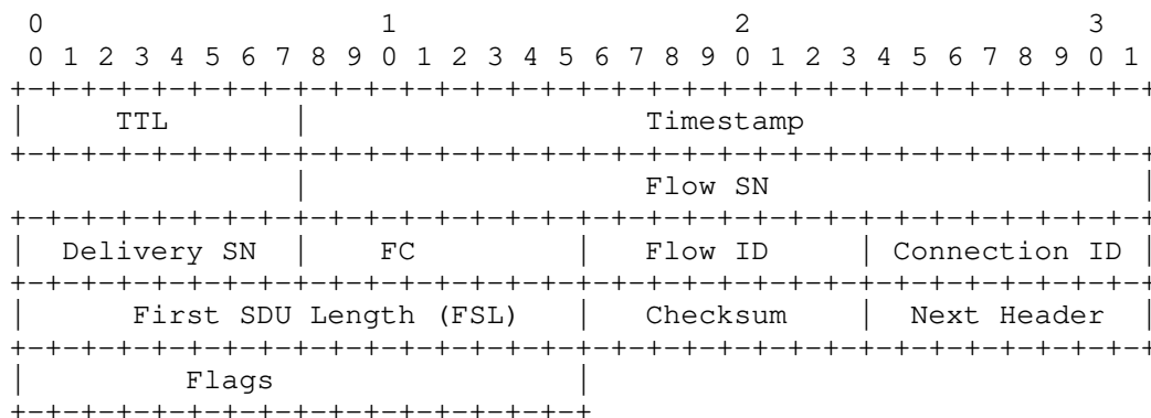
Figure 4: GMA Trailer Format with All Optional Fields Present
