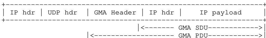
Figure 7: GMA PDU Format with Non-IP Encapsulation
