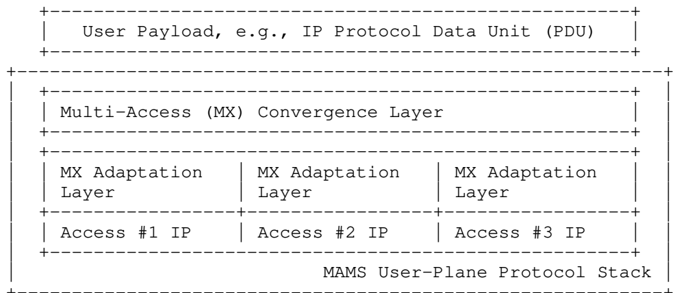
Figure 1: MAMS User-Plane Protocol Stack
