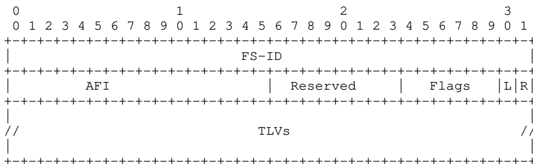
Figure 2: PCEP FLOWSPEC Object Body Format
