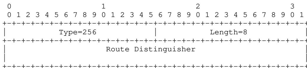
Figure 3: The Format of the ROUTE-DISTINGUISHER TLV
