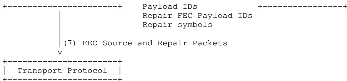
Figure 1: FECFRAME Architecture at a Sender
