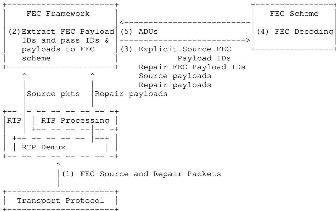
Figure 5: Receiver Operation with Sliding Window FEC Codes and RTP Repair Flows
