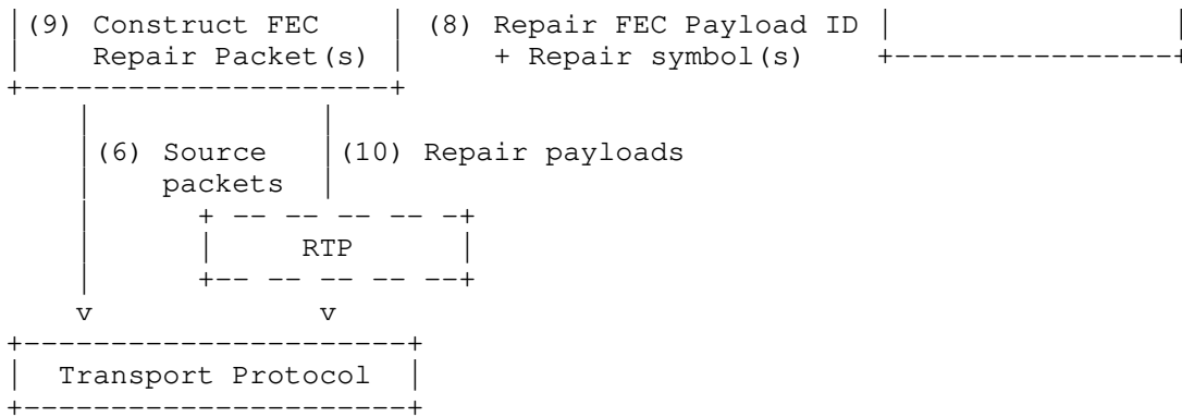
Figure 3: Sender Operation with Sliding Window FEC Codes and RTP Repair Flows
