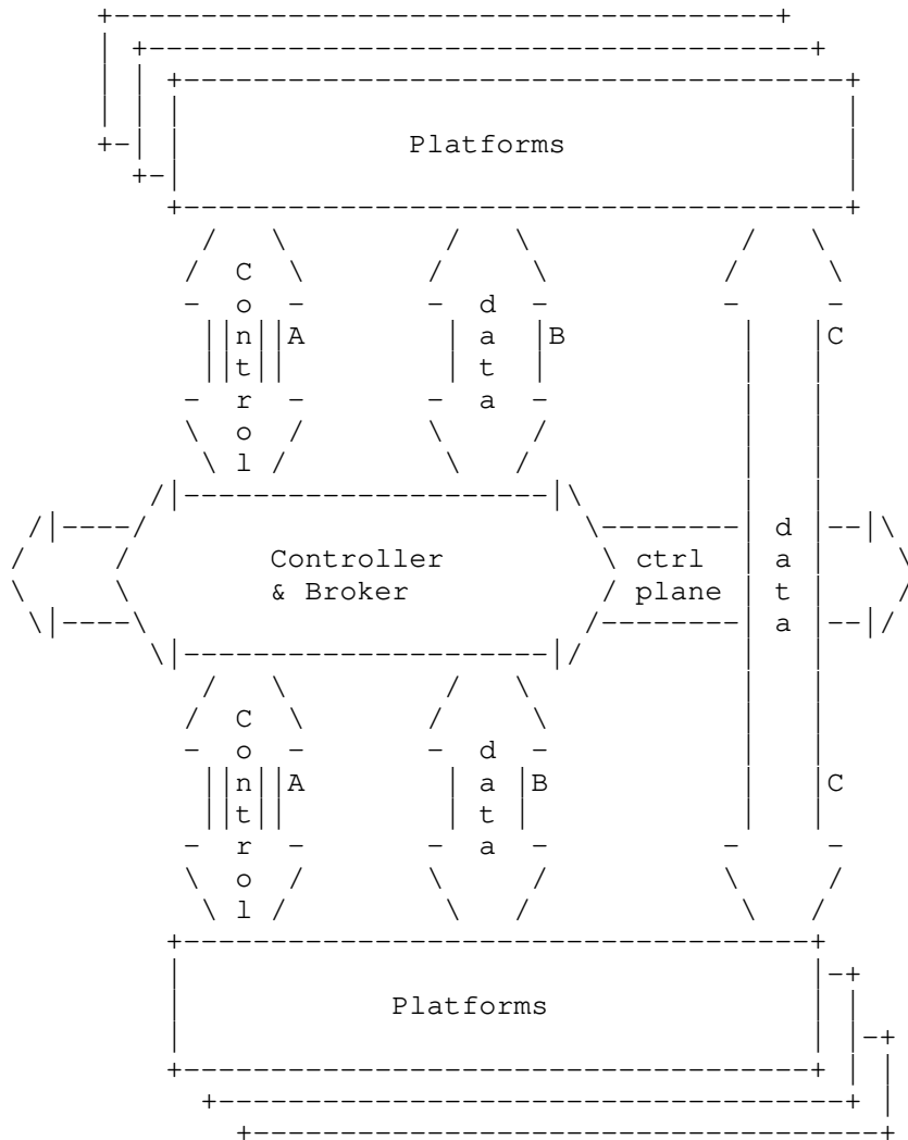
Figure 1: XMPP-Grid Architecture
