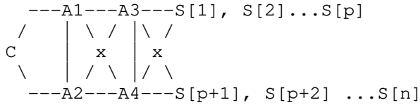
Figure 13: Full Mesh
