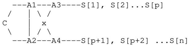
Figure 12: Agent Chains
