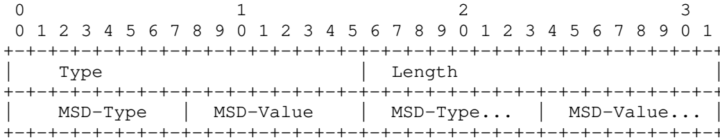
Figure 2: Link MSD Sub-TLV
