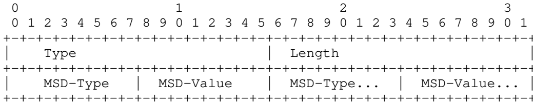
Figure 1: Node MSD TLV
