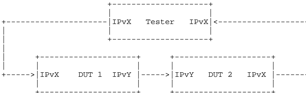
Figure 2: Test Setup 2 (Dual DUT)
