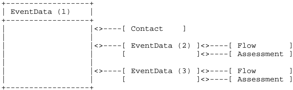
Figure 30: Recursion in the EventData Class
