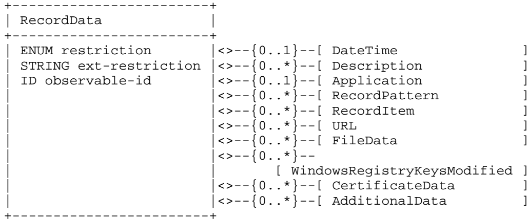
Figure 46: The RecordData Class
