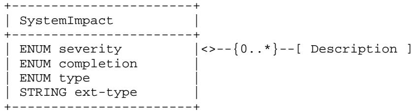
Figure 22: The SystemImpact Class
