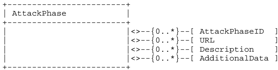
Figure 73: The AttackPhase Class
