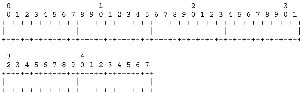
Figure 1: Value Field of the "Additional PMSI Tunnel Attribute Flags" Extended Community
