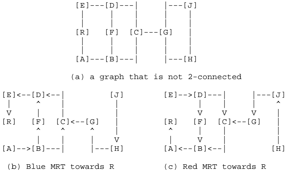
Figure 2: A Network That Is Not 2-Connected
