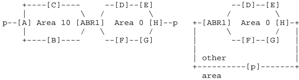
(a) Example topology (b) Proxy node view in Area 0 nodes
