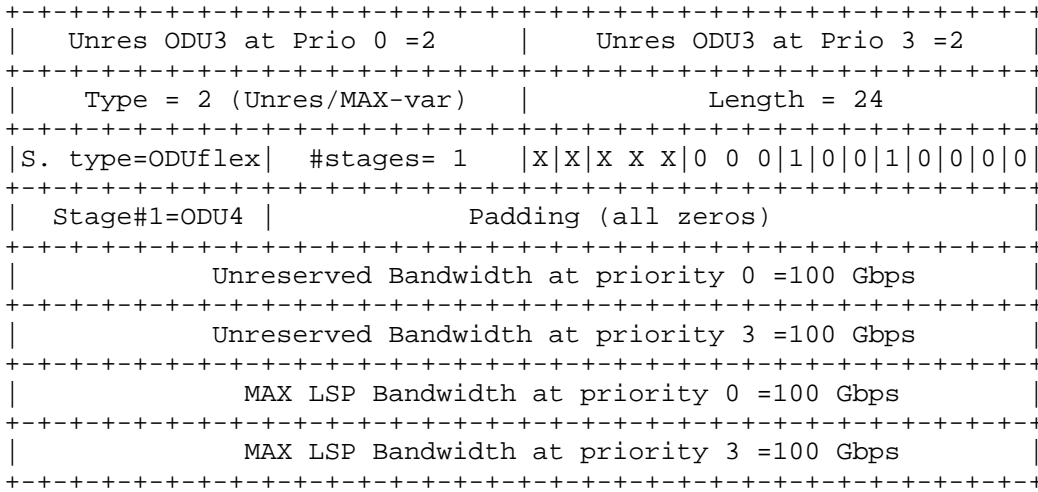
Figure 13: Single-Stage Muxing
