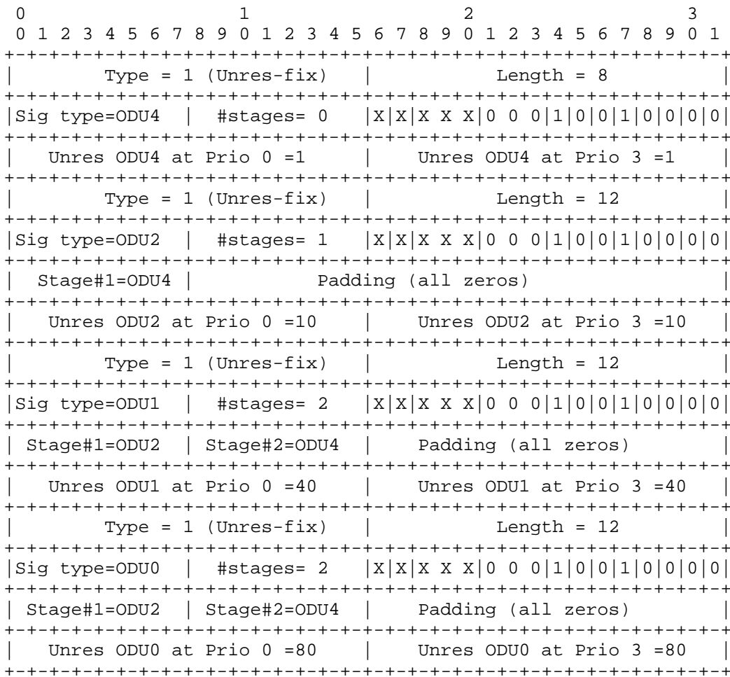
Figure 17: Multi-Stage Muxing -- Non-Homogeneous Hierarchies -- ISCD 2
