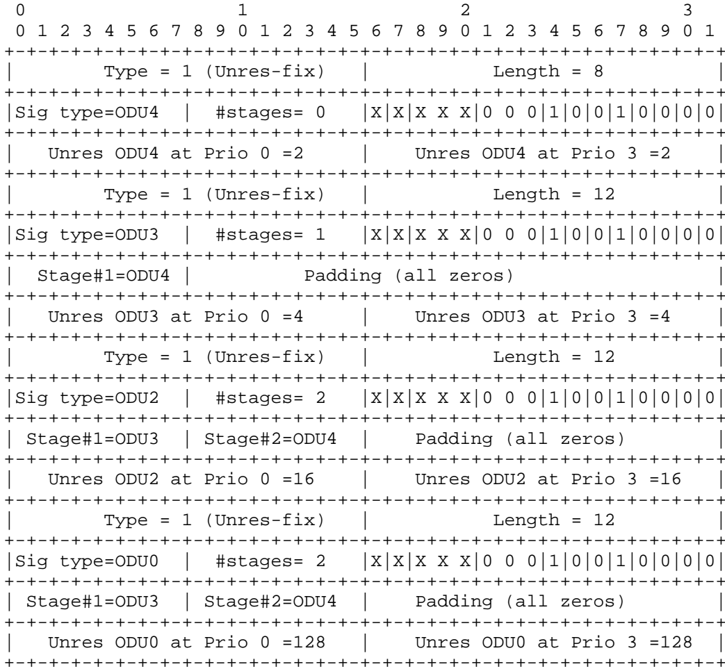
Figure 15: Multi-Stage Muxing -- Bundled Links
