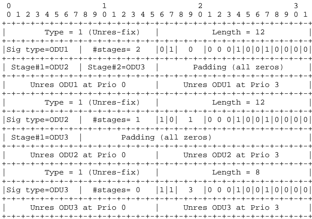
Figure 10: Utilization of Different TS Granularities -- ISCD 2
