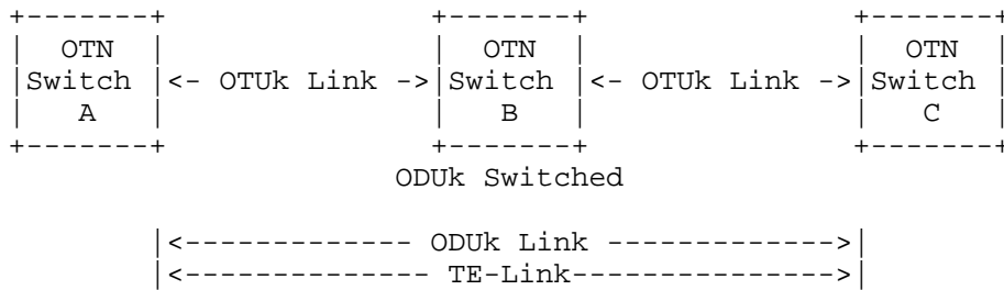
Figure 2: Multiple-Hop TE-Link
