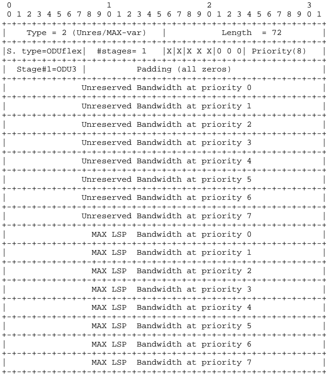
Figure 12: ODUflex Advertisement
