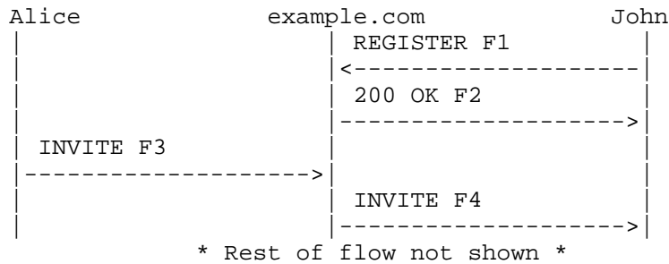
Figure 5: Alias Example
