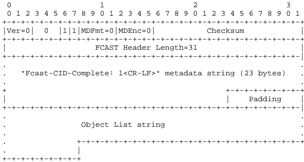
Figure 5: CID Object Example: Static Session
