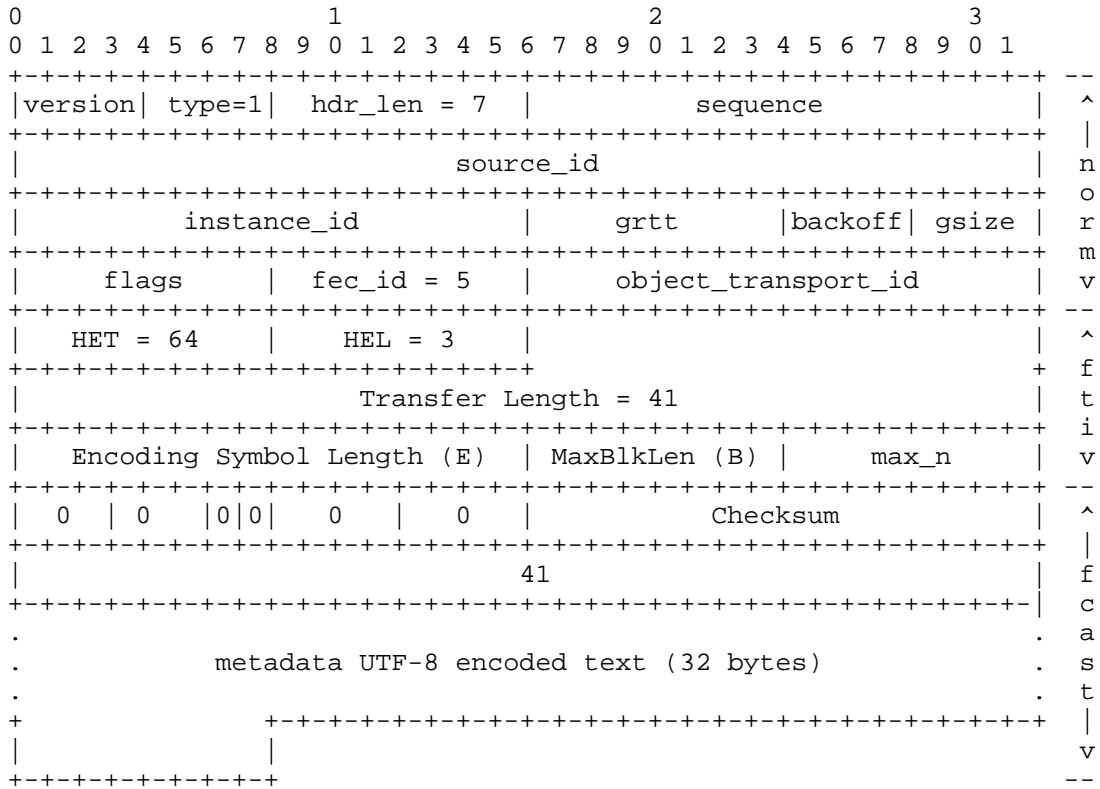
Figure 6: NORM_INFO Message Containing an EXT_FTI Header Extension and an FCAST Header
