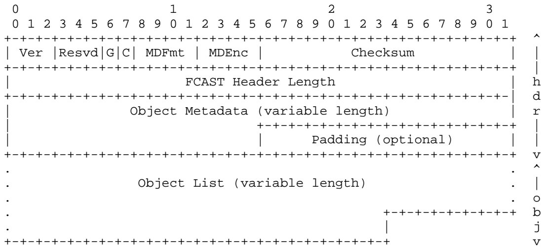
Figure 2: Carousel Instance Descriptor Format
