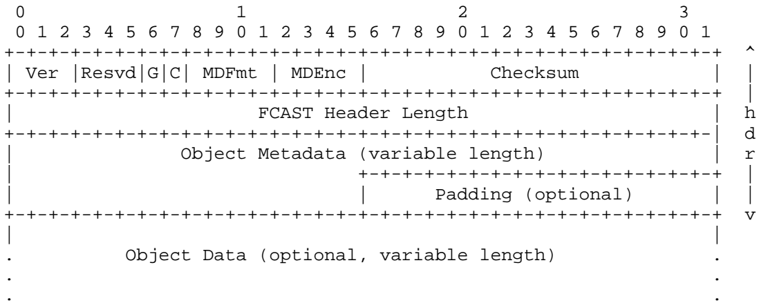
Figure 1: Compound Object Format
