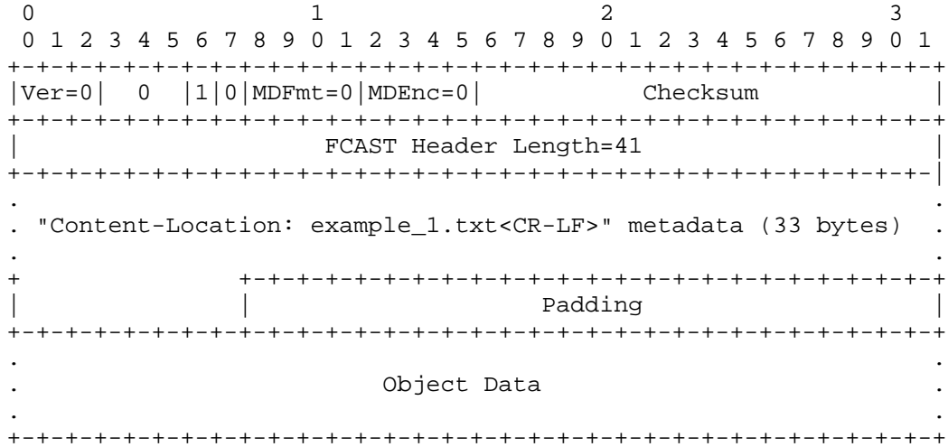
Figure 4: Simple Compound Object Example
