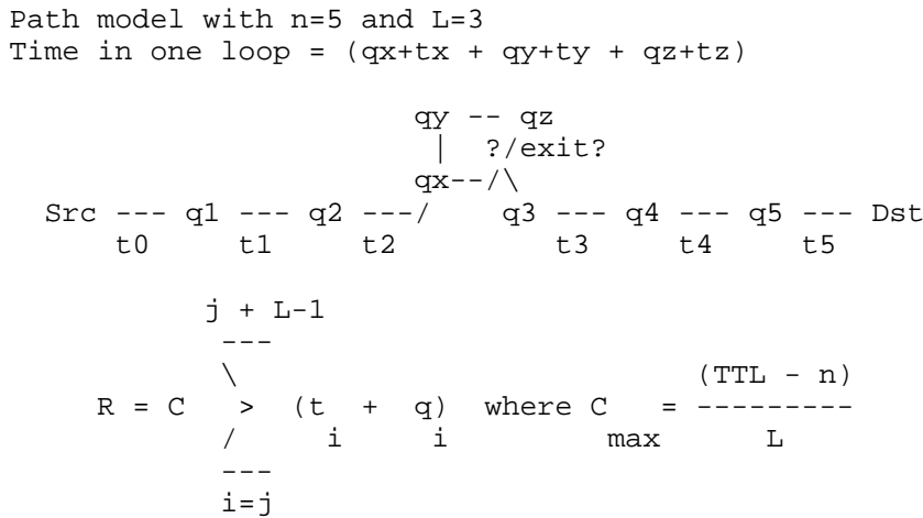
Figure 2: Delay Due to Rotations in a Loop
