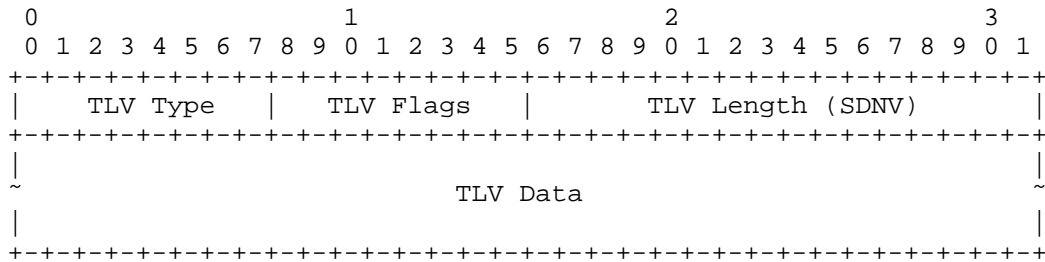
Figure 6: TLV Format
