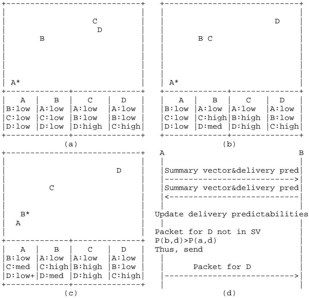
Figure 13: PROPHET example
