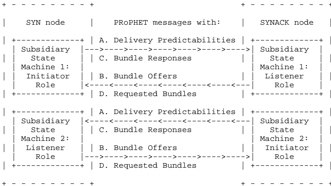
Figure 12: Information Exchange Phase Subsidiary State Machines
