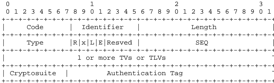
Figure 6: EAP-Initiate/Re-auth Extension
