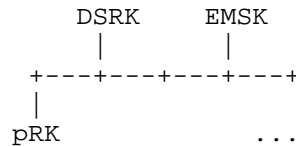
Figure 3: ERP/AAK Root Key Derivation
