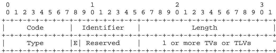
Figure 5: EAP-Initiate/Re-auth-Start Extension
