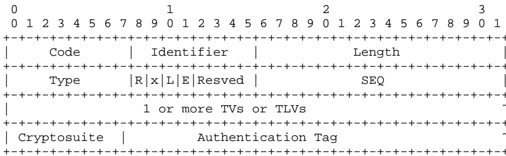
Figure 7: EAP-Finish/Re-auth Extension
