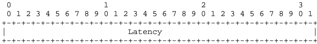
Figure 9: Latency Sub-Object Format
