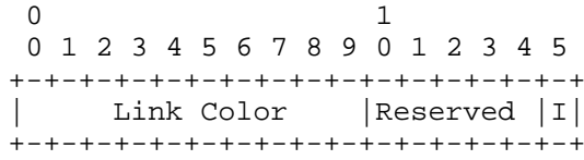
Figure 16: LC Type 2 Sub-Object Format
