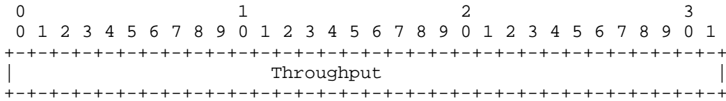
Figure 7: Throughput Sub-Object Format
