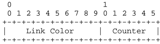
Figure 15: LC Type 1 Sub-Object Format
