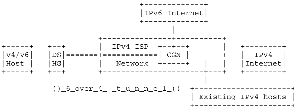
Figure 1: Incremental CGN Approach with IPv4 ISP Network
