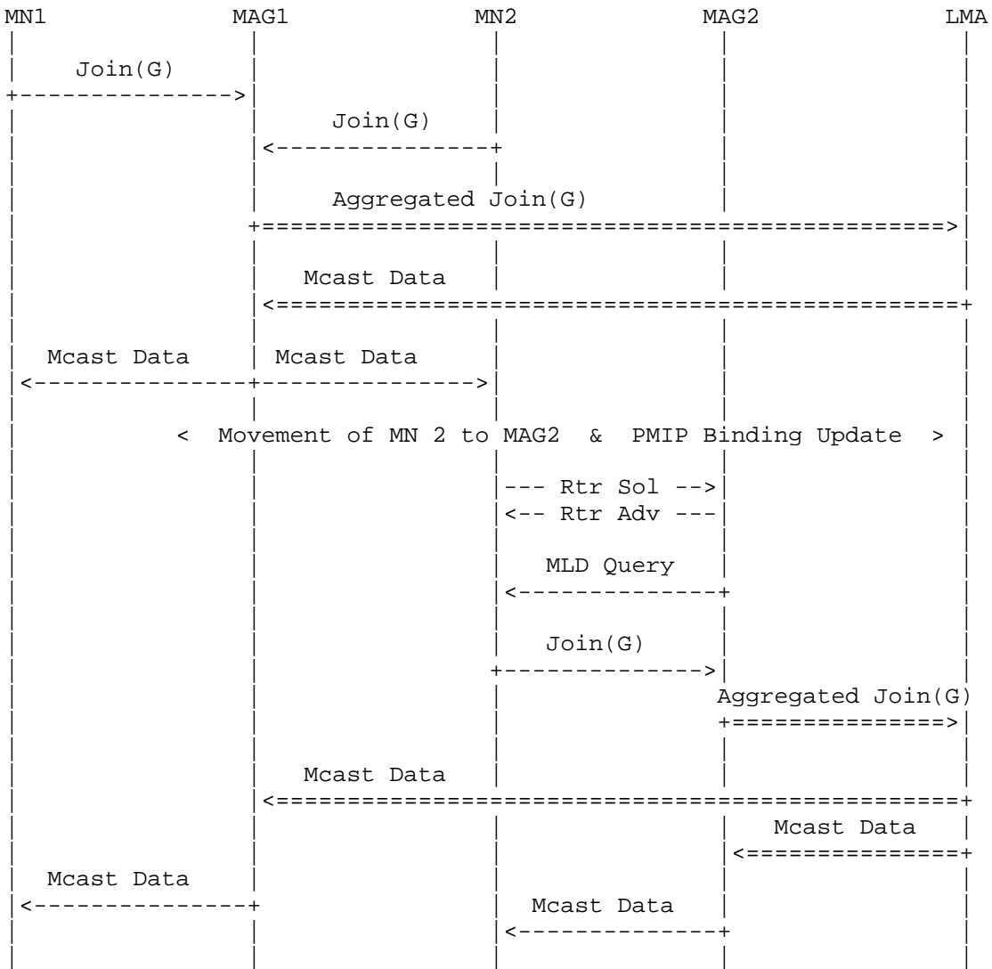
Figure 2: Call Flow of Multicast-Enabled PMIP with "MLD Membership Report" Abbreviated by "Join"
