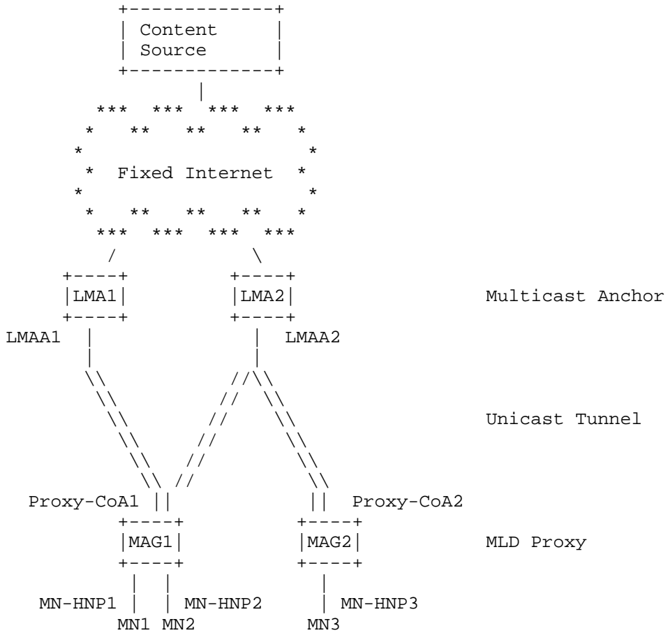
Figure 1: Reference Network for Multicast Deployment in PMIPv6
