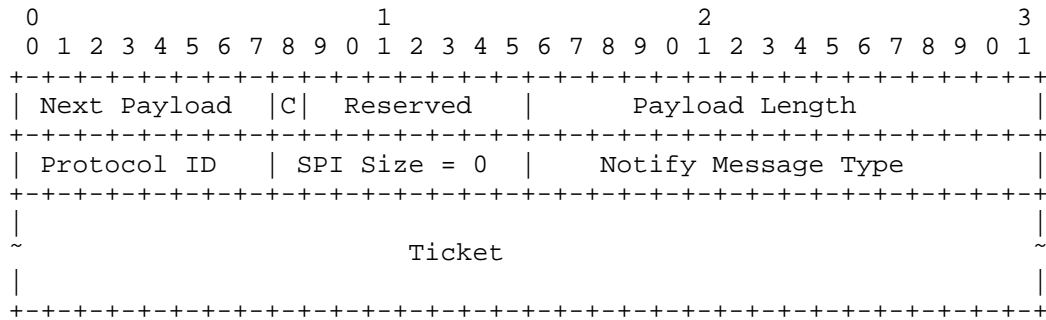
Figure 7: TICKET_OPAQUE Notify Payload
