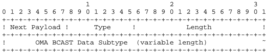
Figure 1: OMA BCAST MIKEY General Extension
