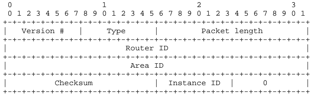
The OSPF Packet Header
