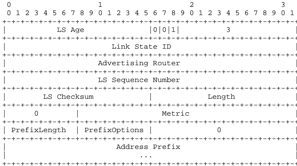
Inter-Area-Prefix-LSA Format
