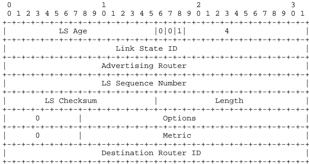
Inter-Area-Router-LSA Format
