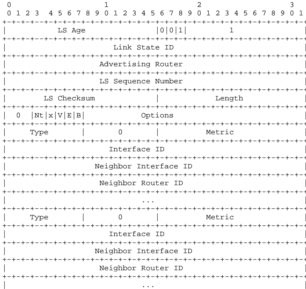
Router-LSA Format
