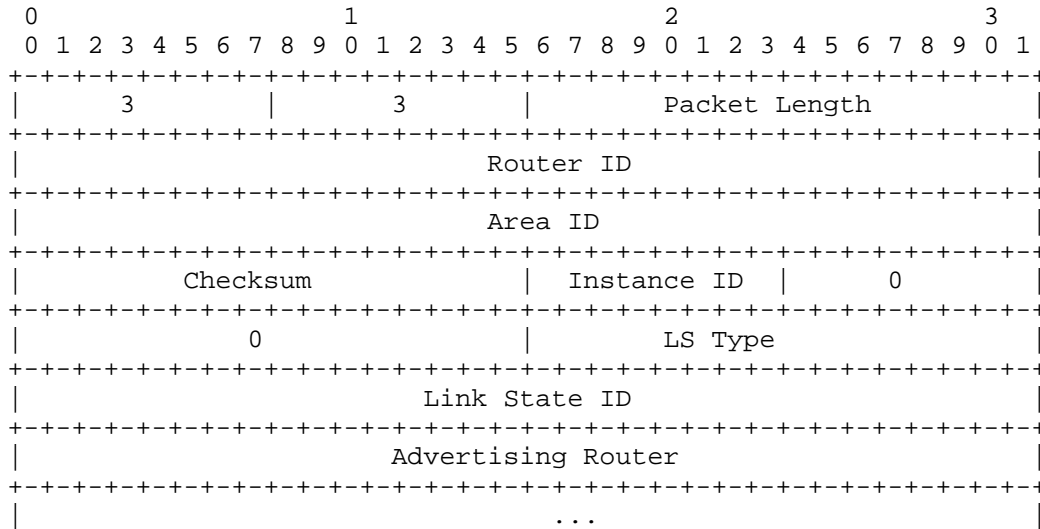
The OSPF Link State Request Packet
