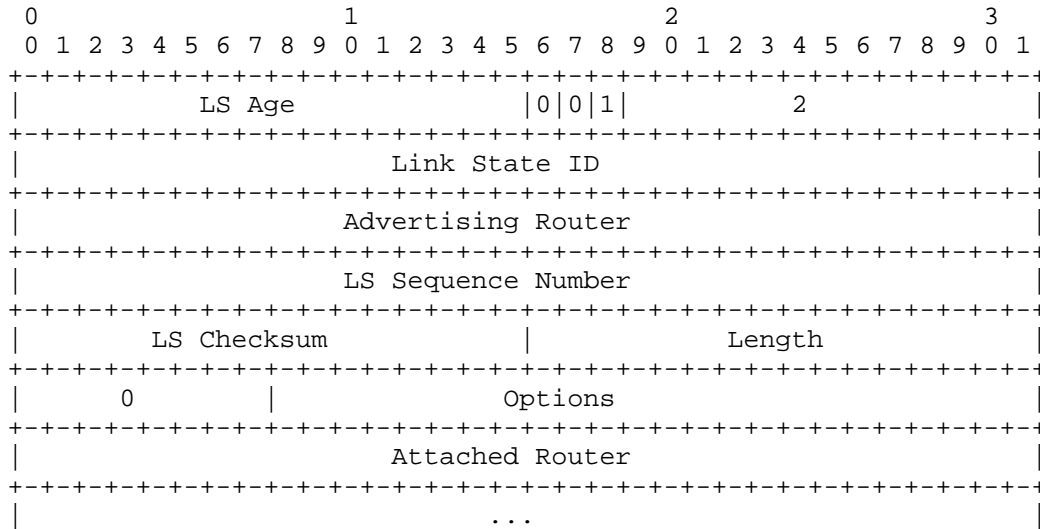
Network-LSA Format
