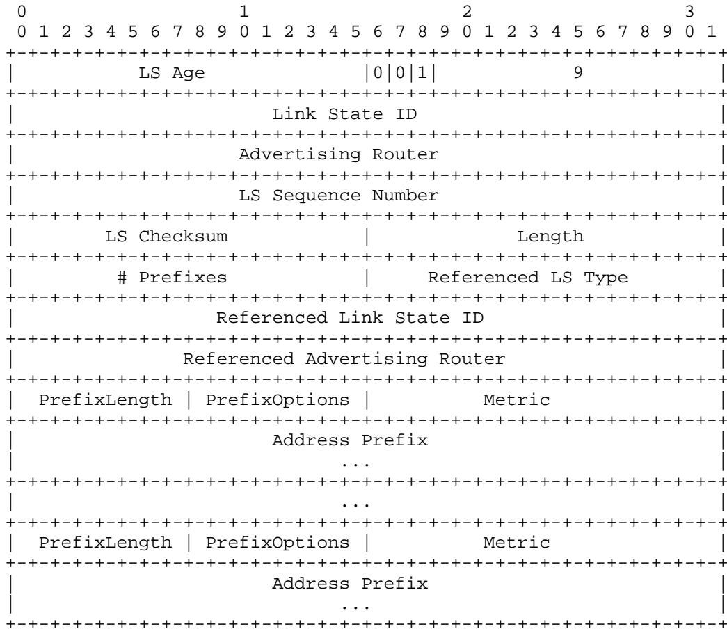
Intra-Area-Prefix LSA Format
