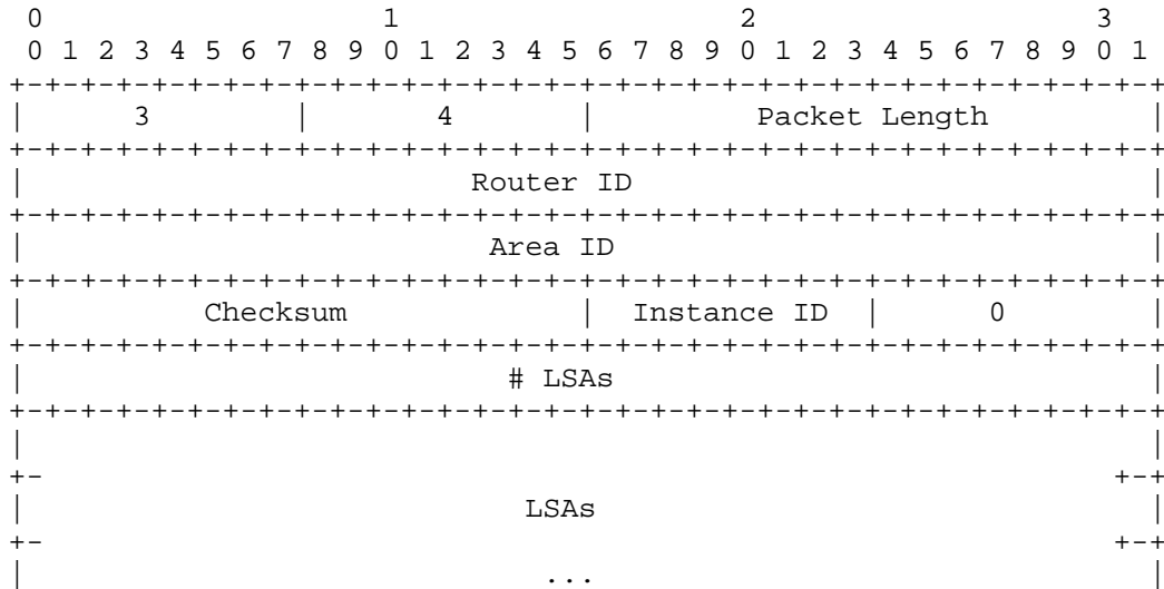
The OSPF Link State Update Packet
