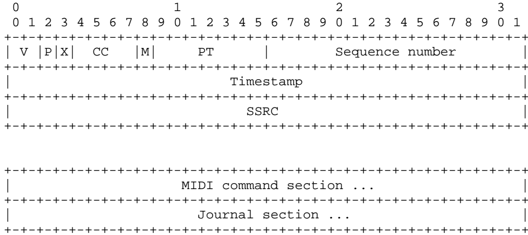
Figure 1 -- Packet format
