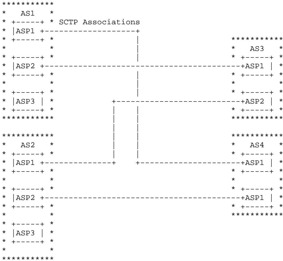
Figure 3: Generalized Architecture
