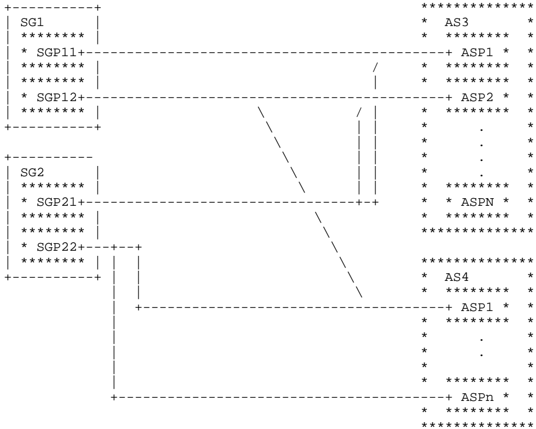
Figure 4: Signalling Gateway Architecture
