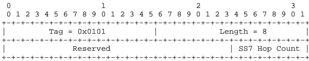
SS7 Hop Counter (3.18/Q.713)
