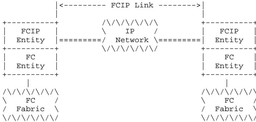
Figure 3: Model for Two Connected FC/FCIP Entity Pairs
