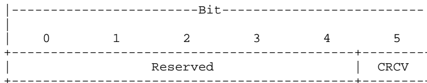
Figure 3 - Flags Field Format
