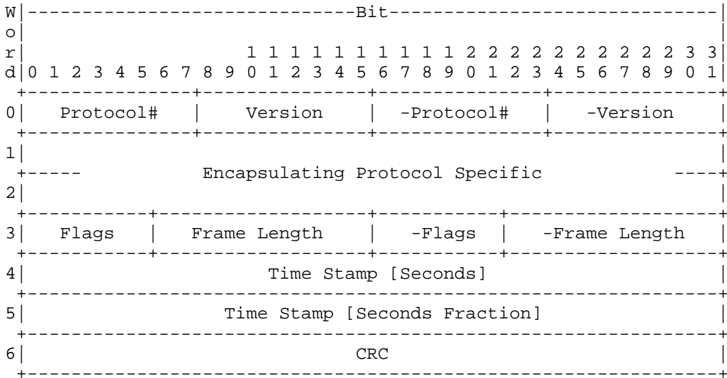
Figure 2 - FC Encapsulation Header Format
