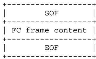
Figure 4 - General FC-2 Frame Format
