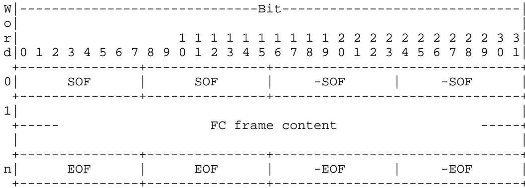
Figure 5 - FC Frame Encapsulation Format
