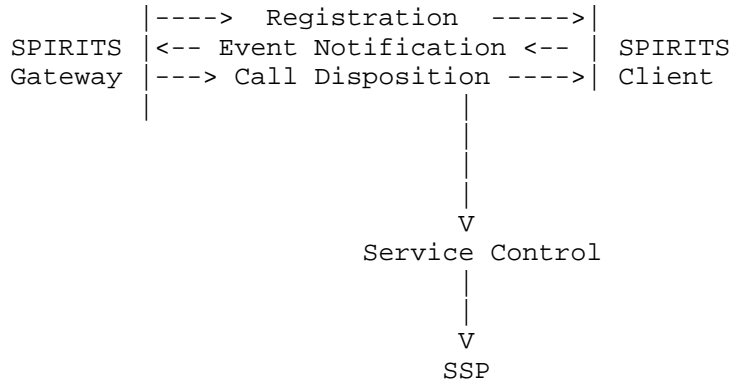
Figure 2: Sequence of SPIRITS actions
