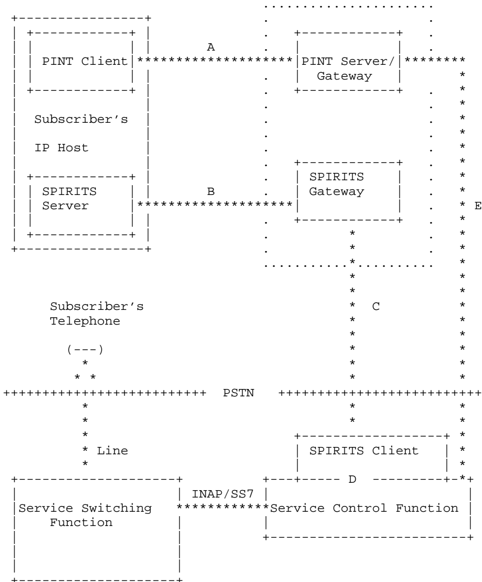
Figure 1. Joint PINT/SPIRITS Architecture
