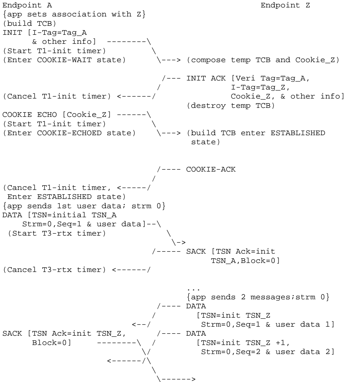
Figure 4: INITiation Example
