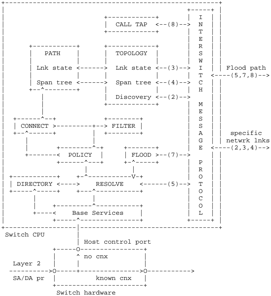
Figure 1: SFVLAN Architectural Overview
