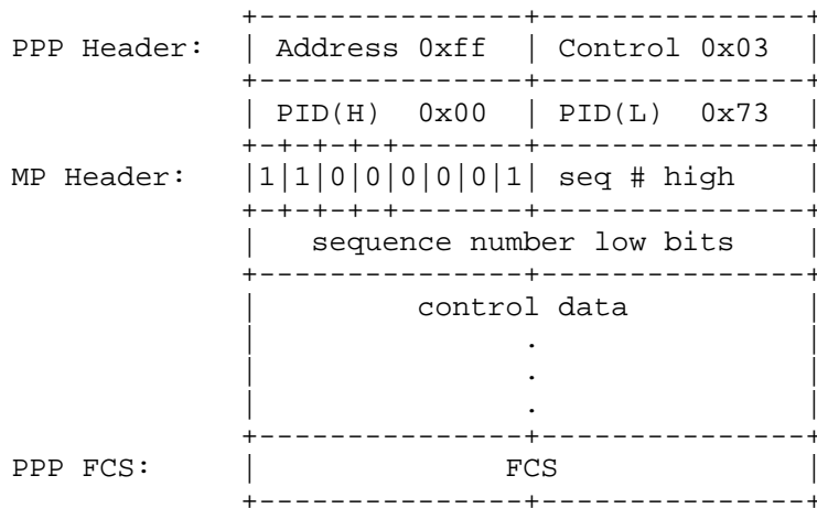
Figure 1: Multilink Plus Frame Format (long sequence number format)
