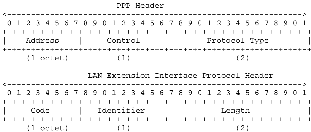
Figure 5 Remote Command Options Frame Format
