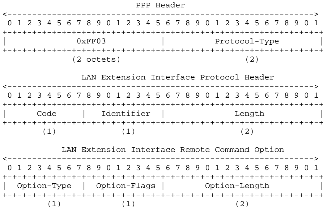
Figure 18 LEX_RCMD_REQUEST Packet Frame Format - Inventory Request
