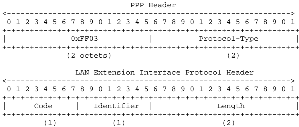
Figure 7 LEX_RCMD_REQUEST Packet Frame Format - Filter MAC Address
