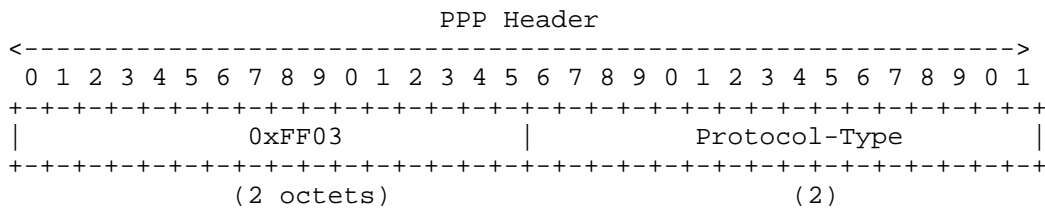
Figure 15 LEX_RCMD_REQUEST Packet Frame Format - Download Data
