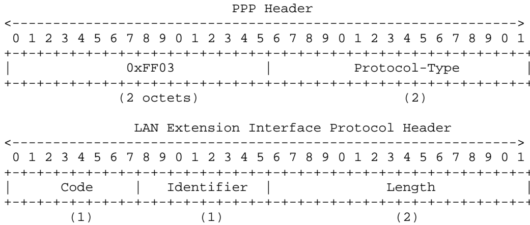
Figure 17 LEX_RCMD_ACK Packet Frame Format - Download Status
