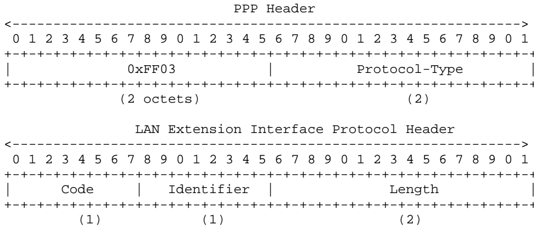
Figure 8 LEX_RCMD_REQUEST Packet Frame Format - Set Priority
