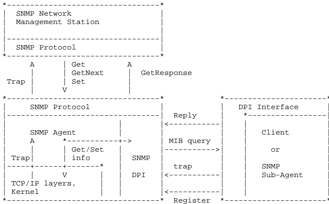
Figure 1. SNMP DPI overview
