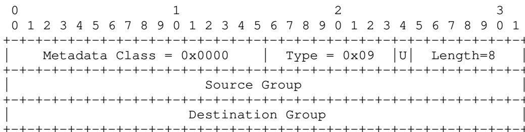
Figure 13: Source/Destination Groups
