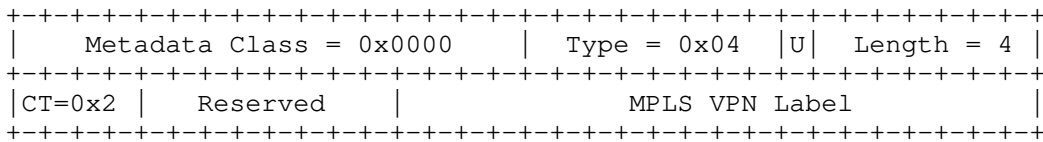
Figure 5: MPLS VPN Forwarding Context
