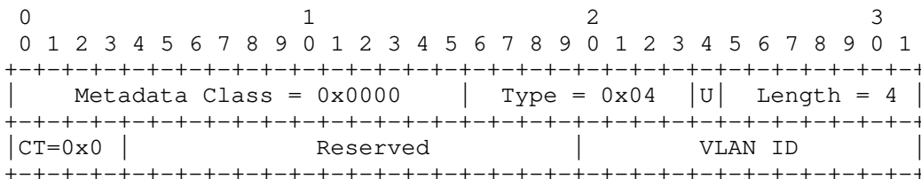
Figure 3: VLAN Forwarding Context
