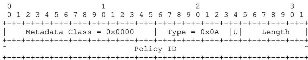
Figure 14: Policy ID
