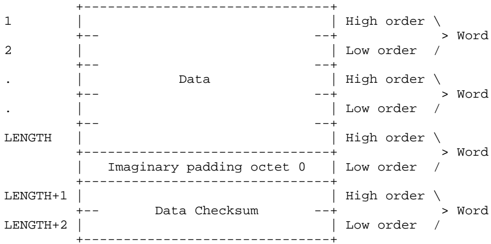
Data Portion of a Packet
