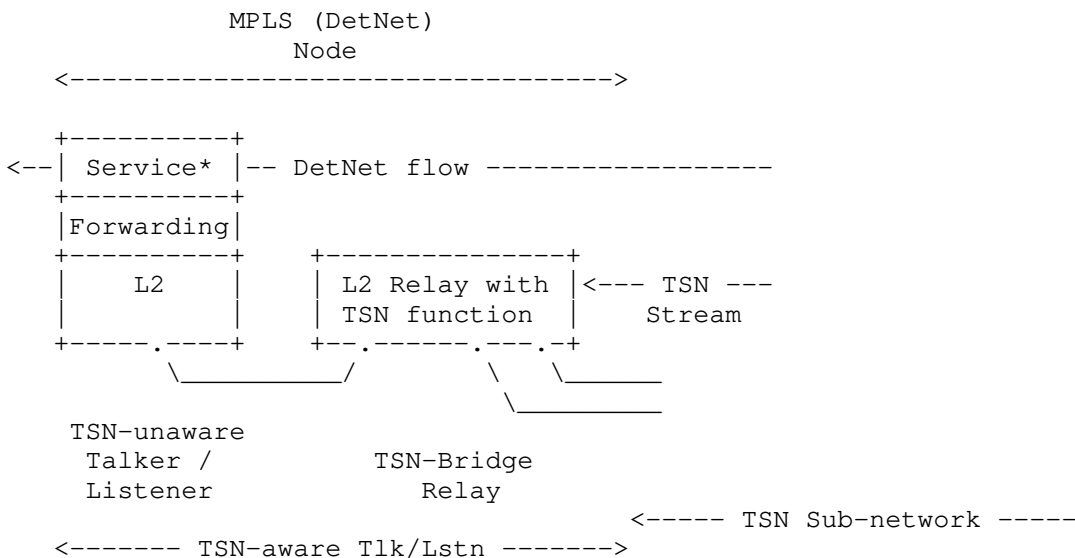
Figure 2: MPLS (DetNet) Node with TSN Functions
