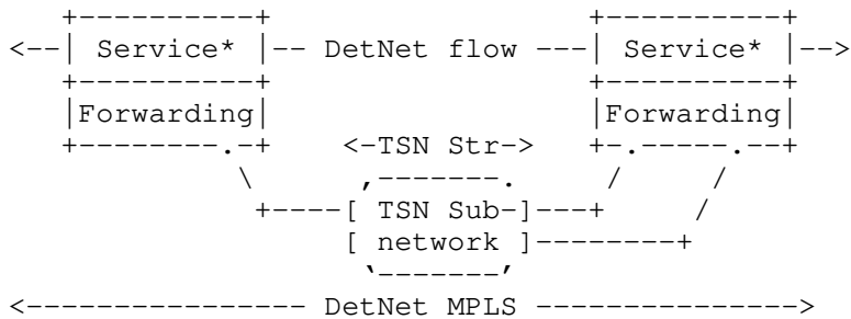
Figure 1: DetNet-Enabled MPLS Network over a TSN Sub-network
