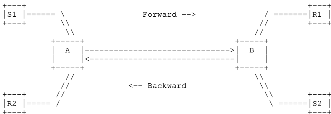
Figure 4: Testbed Topology for Congested Feedback Link
