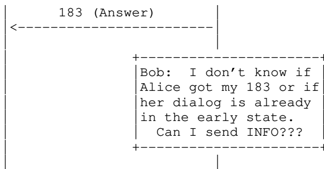
Figure 4: A SIP UA that sent an Answer in an unreliable provisional response does not know if it was received or if the dialog at the side of the Offerer has entered the early state
