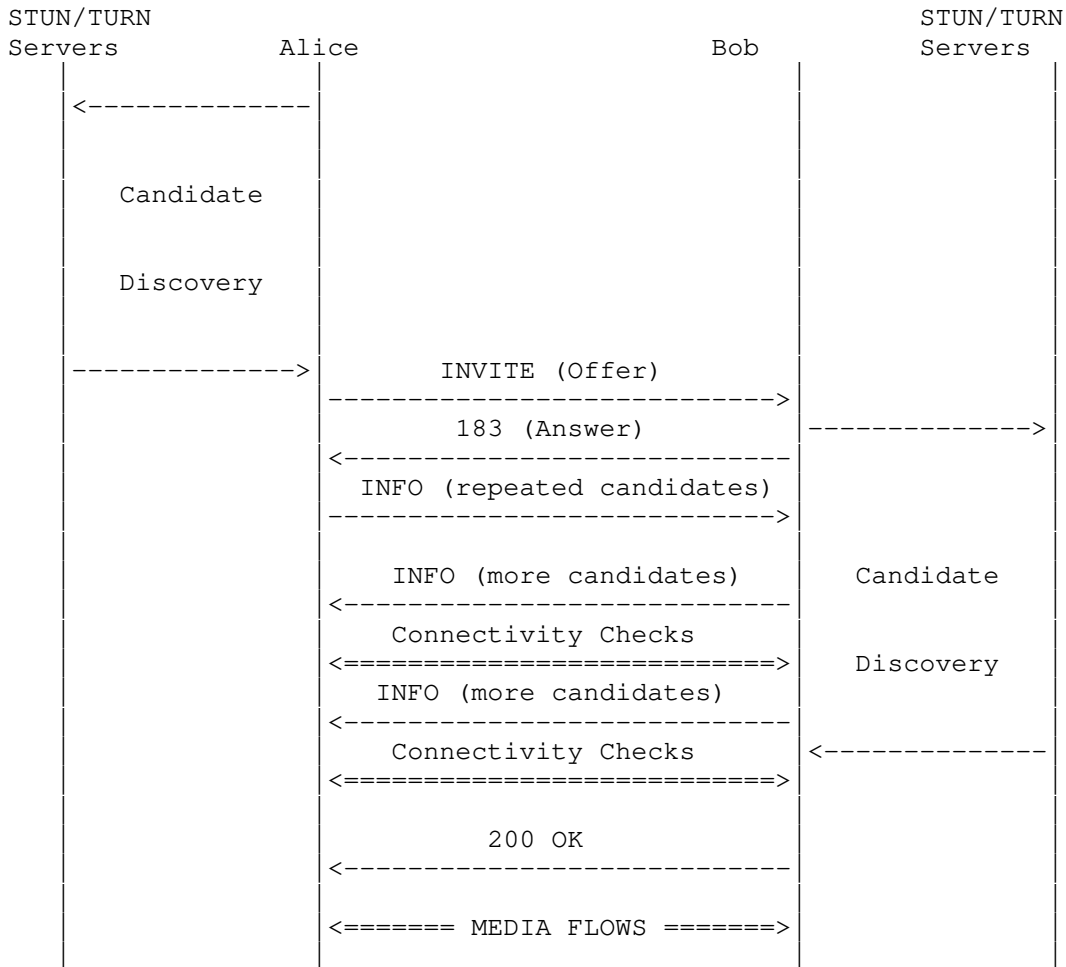
Figure 9: Example of a Typical (Half) Trickle ICE Exchange with SIP
