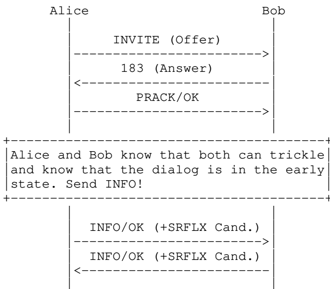
Figure 3: A SIP Offerer can freely trickle as soon as it receives an Answer
