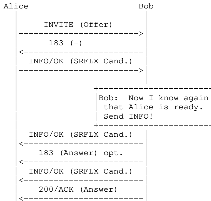
Figure 6: A SIP UA sends an unreliable provisional response without an Answer for establishing an early dialog
