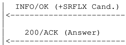
Figure 5: A SIP UA that received an INFO request after sending an unreliable provisional response knows that the dialog at the side of the receiver has entered the early state
