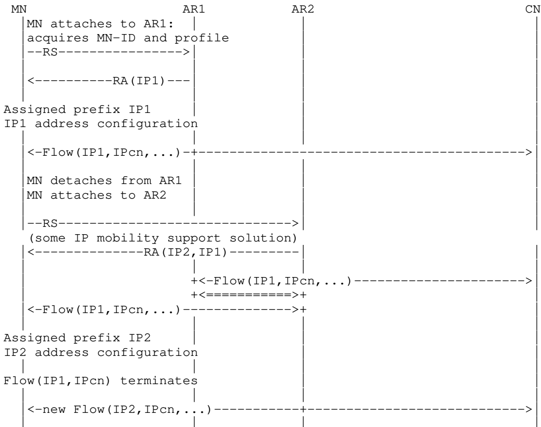
Figure 5: Flow Using IP Prefix from Home Network after MN has Moved
