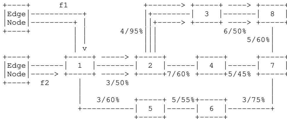
(a) Dijkstra's Algorithm (OSPF/IS-IS)
