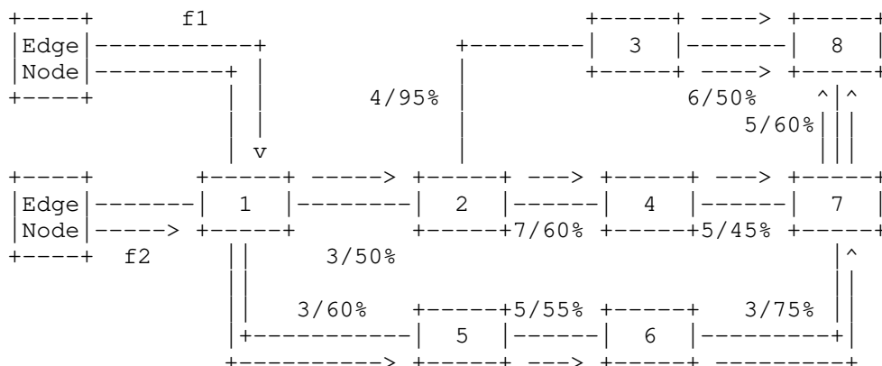
(b) CCDR Algorithm
