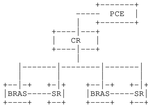
Figure 3: Link Utilization Maximization via CCDR
