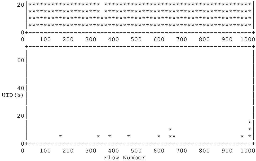
Figure 7: Simulation Results with Congestion Elimination
