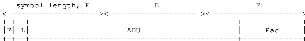
Figure 1: ADUI Creation Example, Resulting in Three Source Symbols
