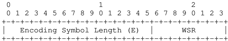
Figure 4: FSSI Encoding Format
