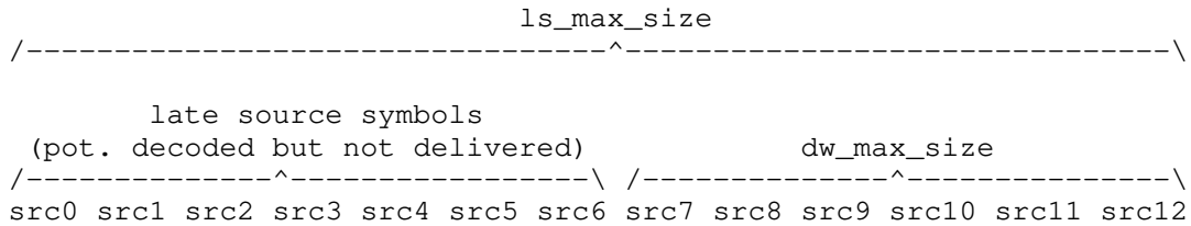
Figure 11: Relationship between Parameters to Decode beyond Maximum Latency
