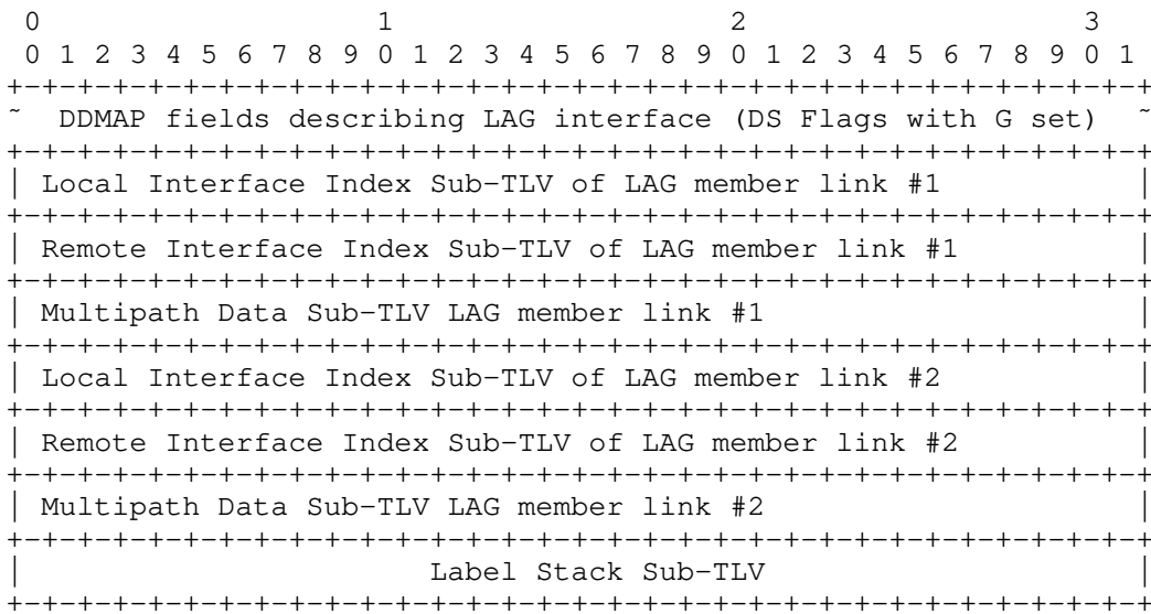
Figure 2: Example of DDMAP in MPLS Echo Reply
