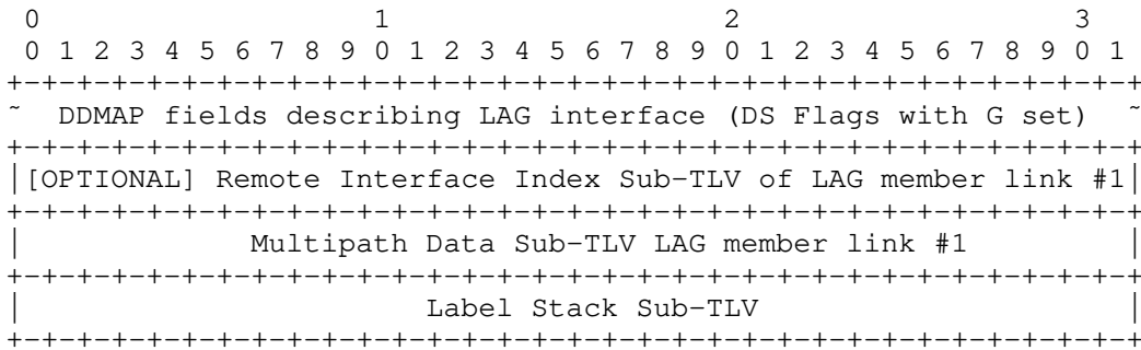
Figure 3: Example of DDMAP in MPLS Echo Request
