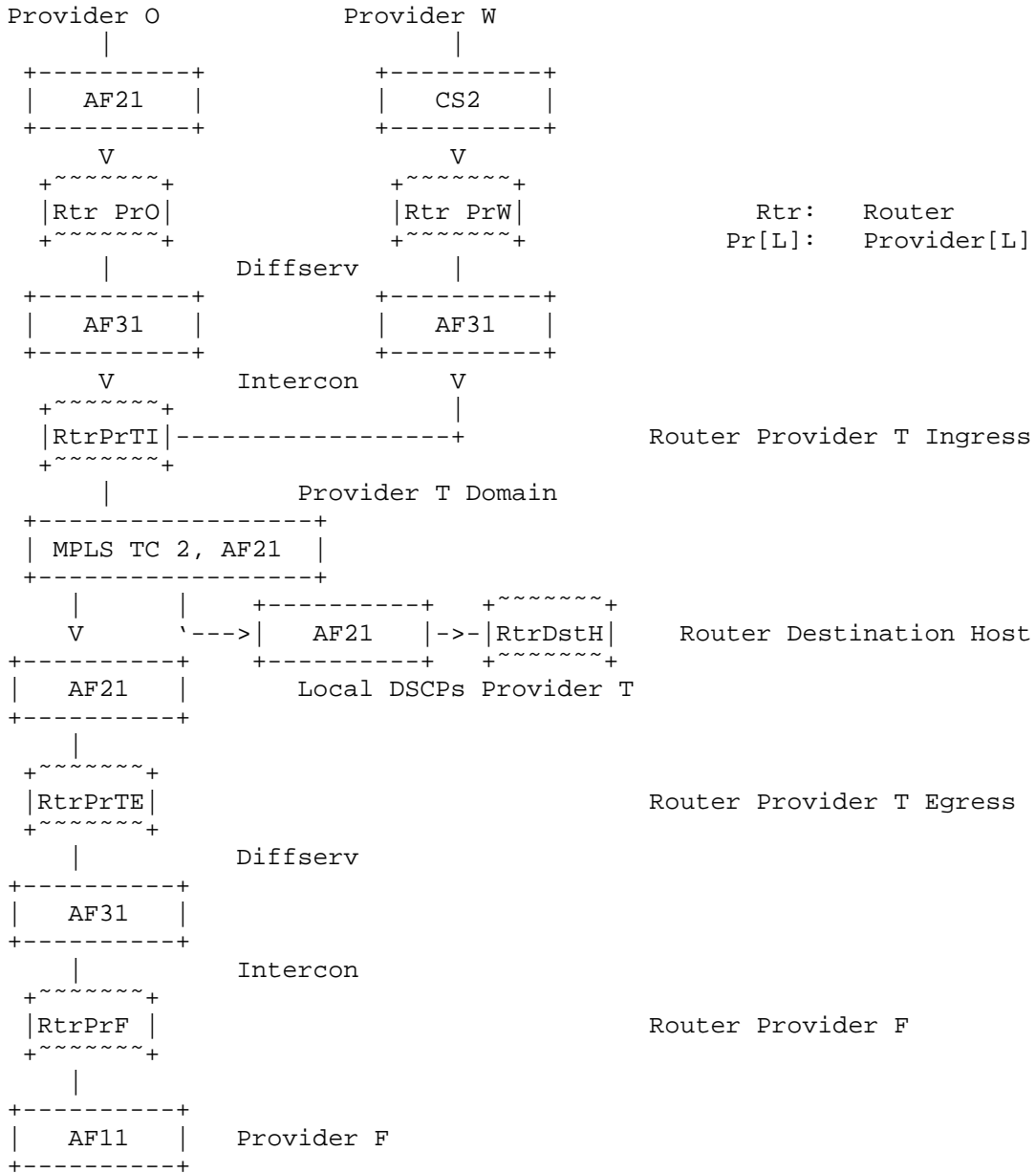
Figure 1: Diffserv-Intercon Example
